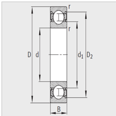
Sealed 2RSR
