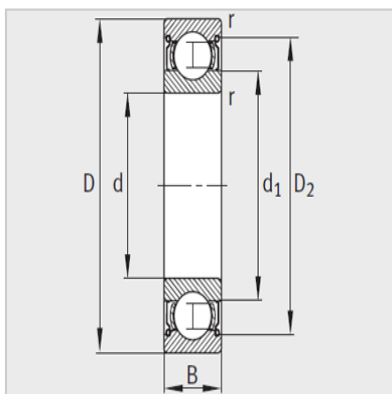
Shields 2Z
